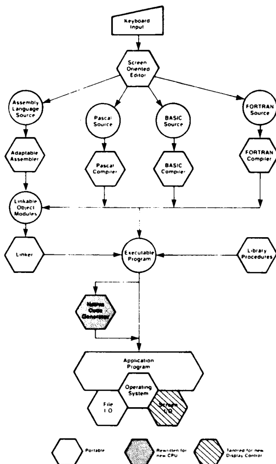
Figure 1-2. Major p-System Components
